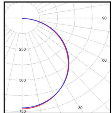
cd/klm — CO-C180 — C90-C270
